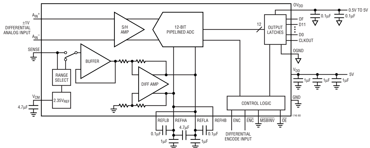
25Msps, 12-Bit ADC with a \pm 1\text{V} Differential Input Range
